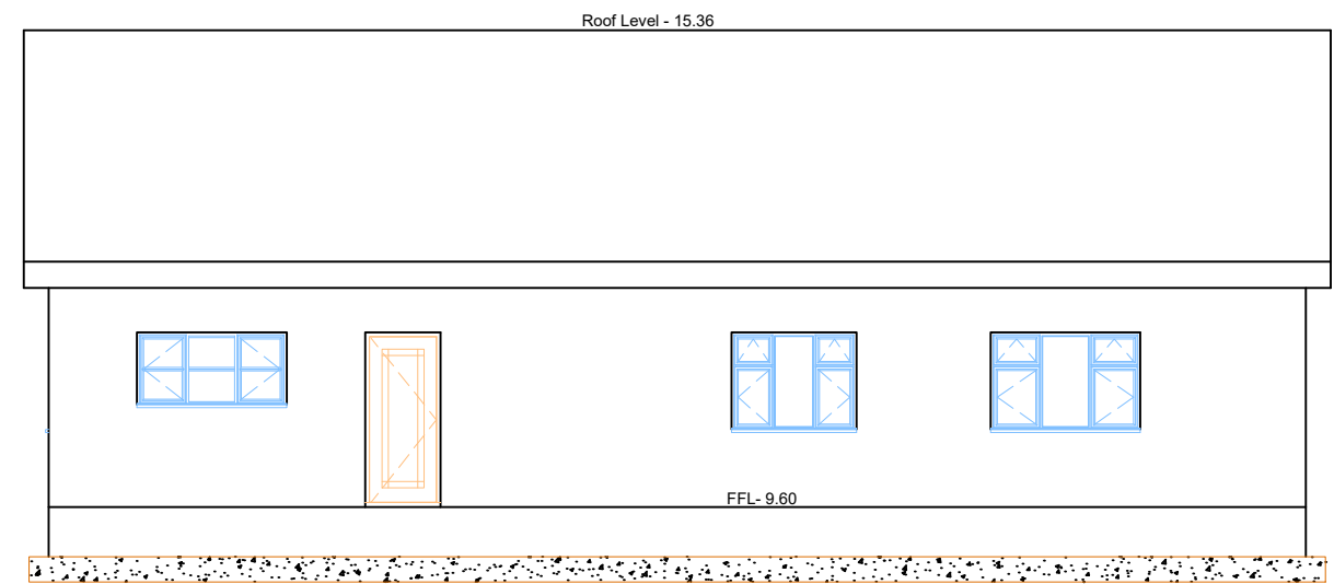
BACK ELEVATION
