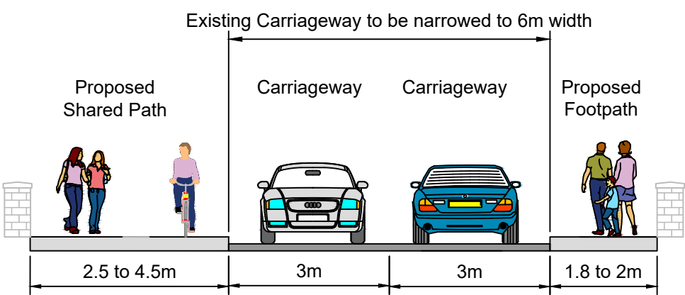
TYPICAL CROSS SECTION A-A SCALE AT A1 1:100
