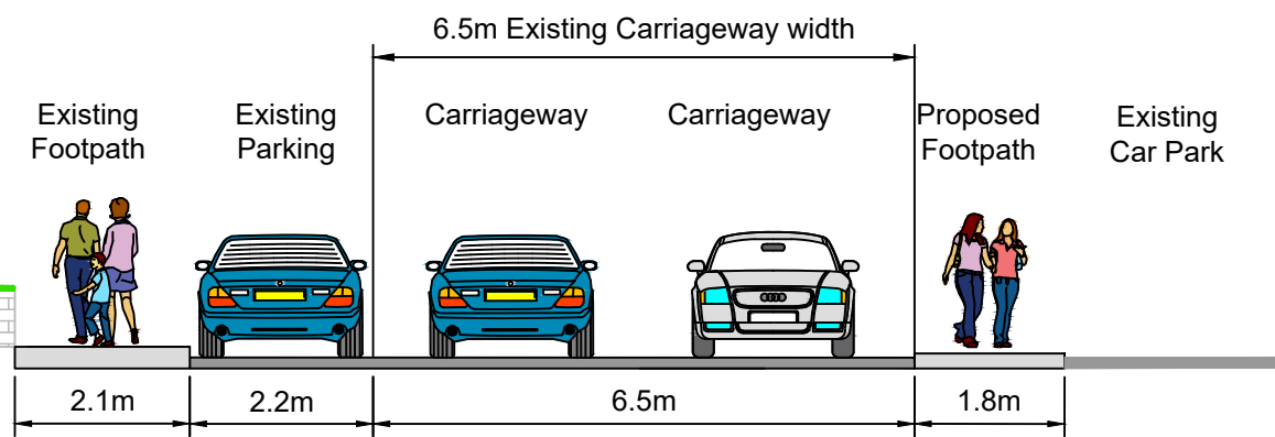
TYPICAL CROSS SECTION E-E SCALE AT A1 1:100
