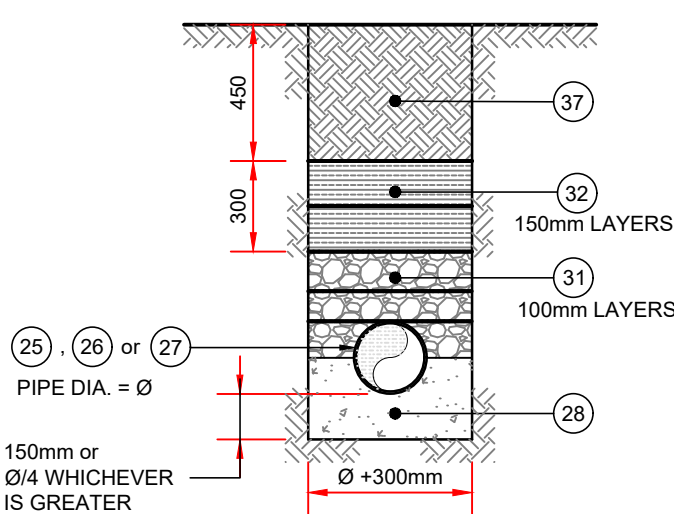
UNDER LANDSCAPED AREAS COVER > 0.9 m
