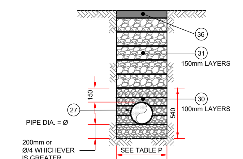
UNDER ROADS/HARDSTANDINGS/FOOTPATHS COVER > 1.2m
