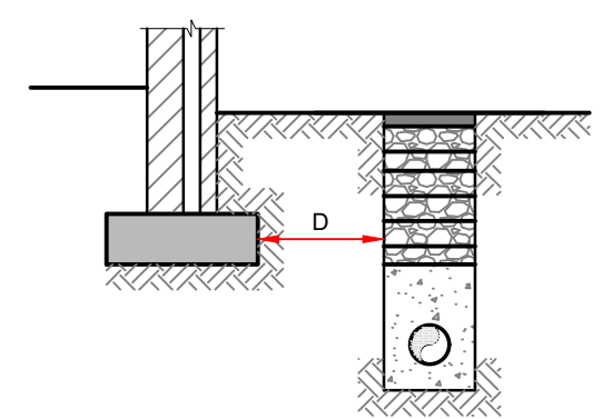
WHERE 'D' IS LESS THAN 1m CONCRETE FILL TO LEVEL OF FOUNDATION BOTTOM)
