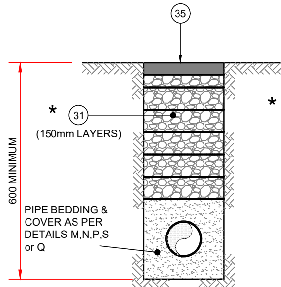
STAGE 1 LEAVE FOR 6 MONTHS TO CONSOLIDATE
