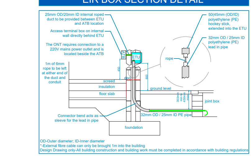
EIR BOX SECTION DETAIL
