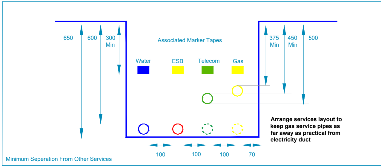
EIR CHAMBER OR JUNCTION BOX
