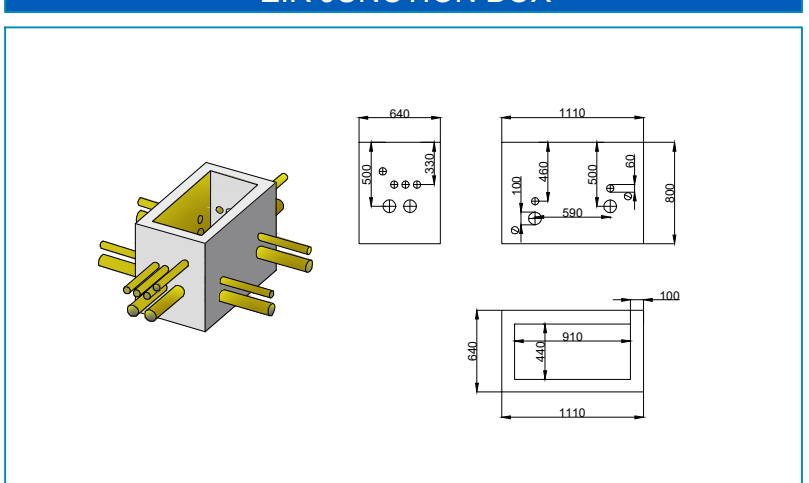
EIR BOX SECTION DETAIL
