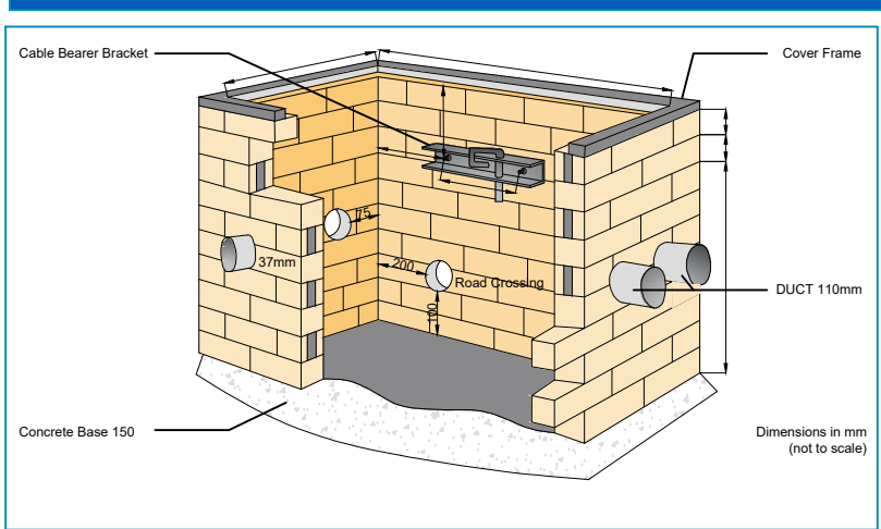
EIR JUNCTION BOX
