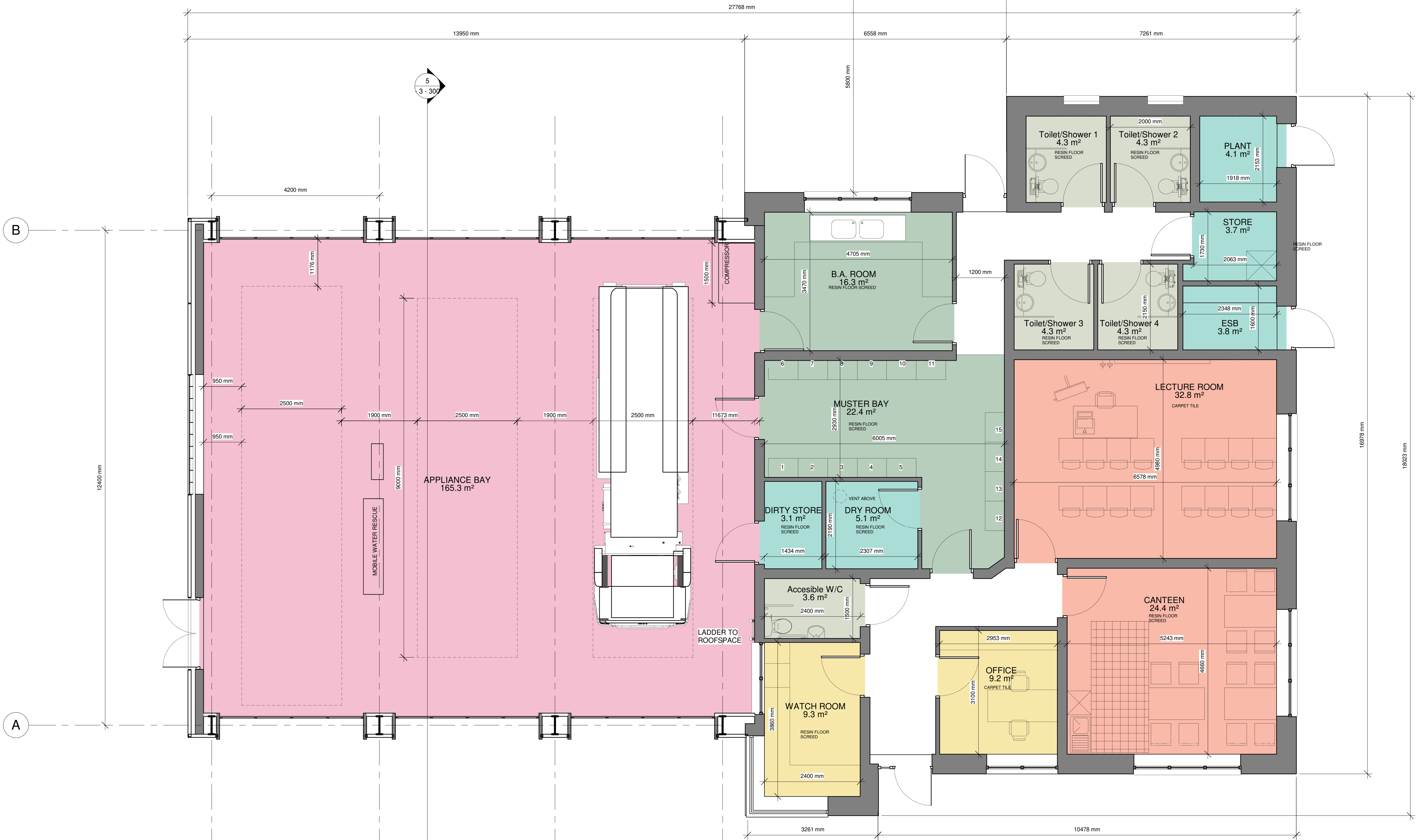
Ground Floor Plan 1:50 @ A1 360.9 sq m
