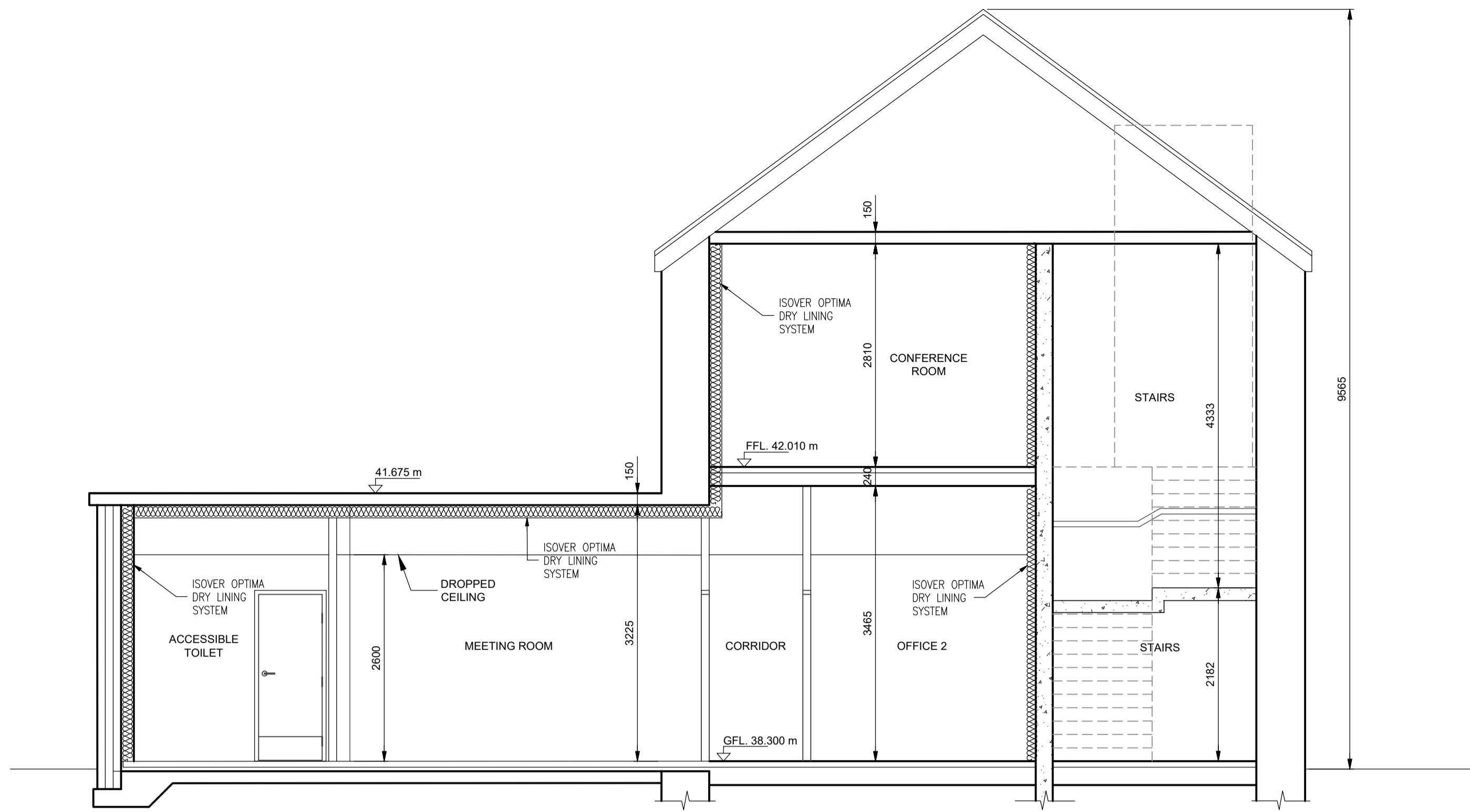
SECTION 1 SCALE 1:50 063/064
