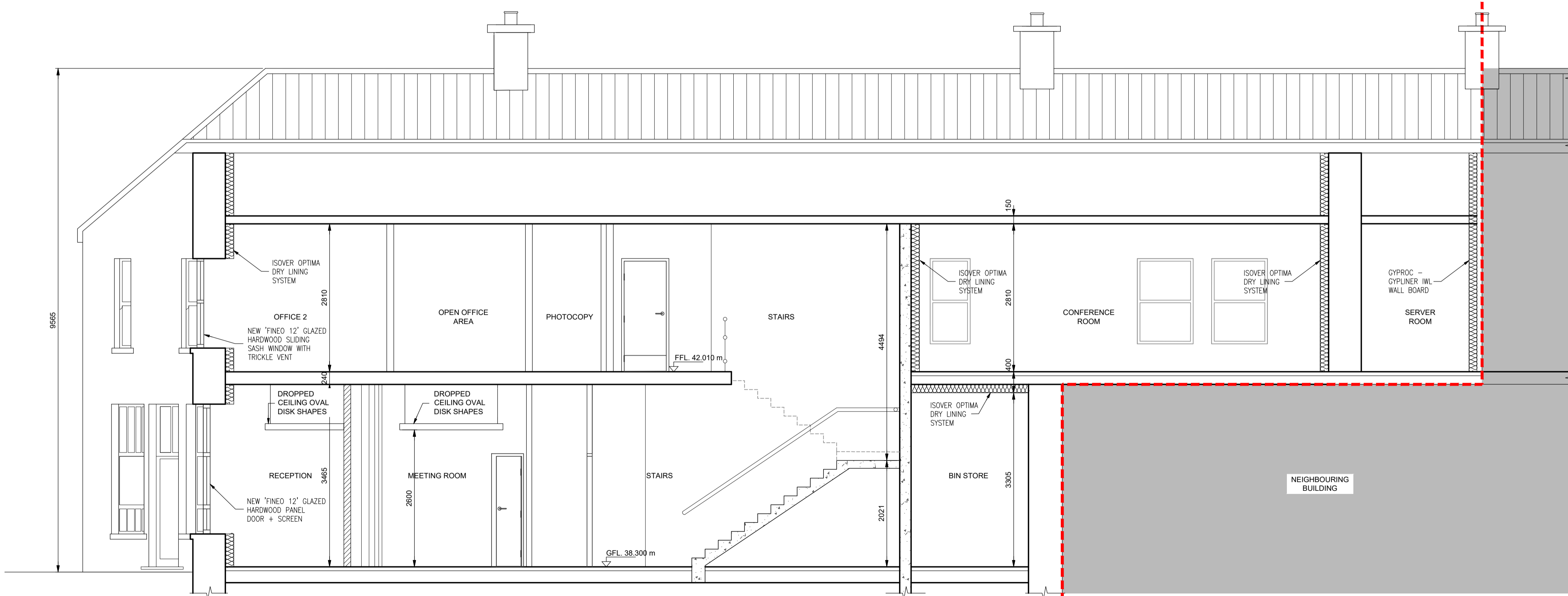
SECTION 2 SCALE 1:50 063/064
