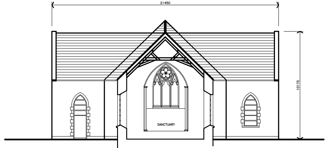
SECTION / WEST ELEVATION Scale 1/50
