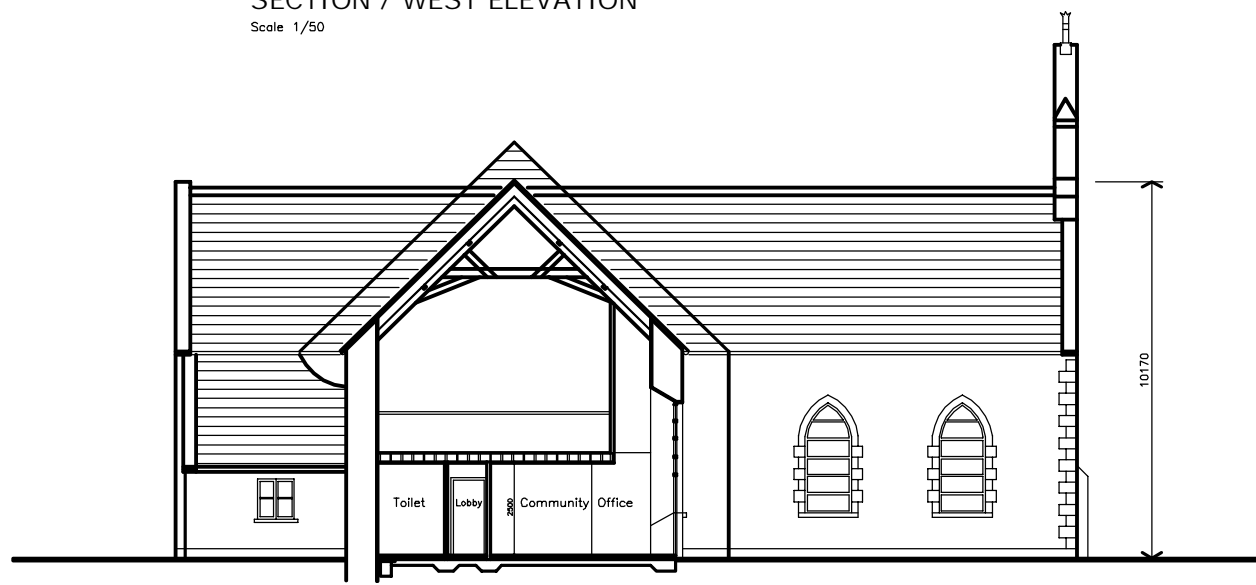
SECTION / NORTH ELEVATION Scale 1/50
