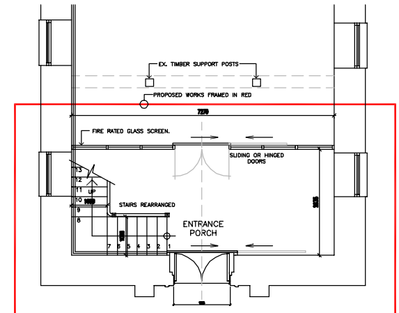
GROUND FLOOR PLAN ENTRANCE LOBBY. PROPOSED.
