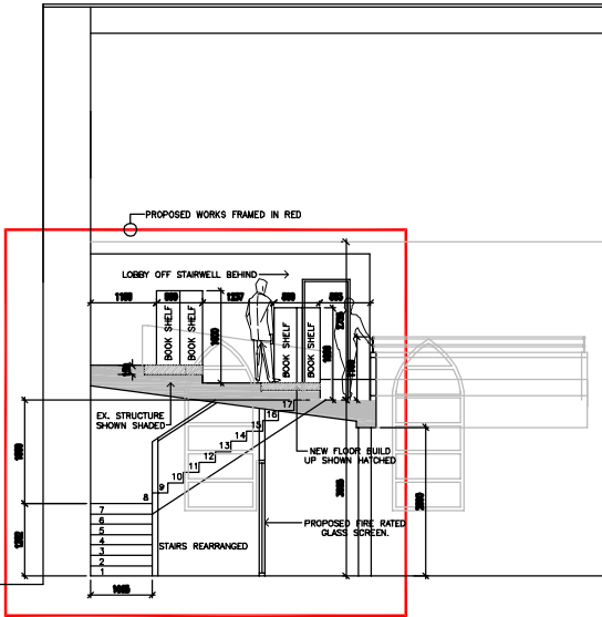
BALCONY CROSS SECTION
