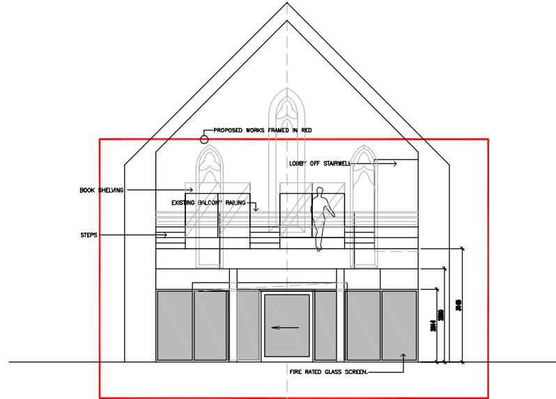
BALCONY SECTION / ELEVATION
