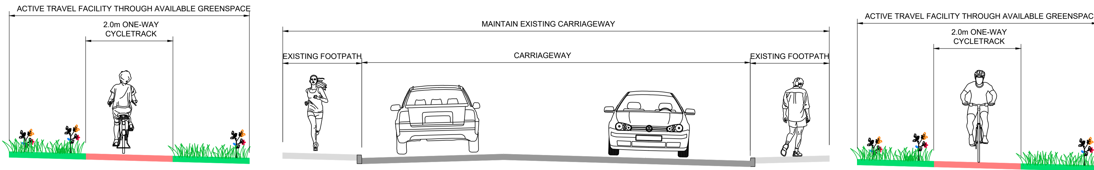
TYPICAL CROSS SECTION B-B
