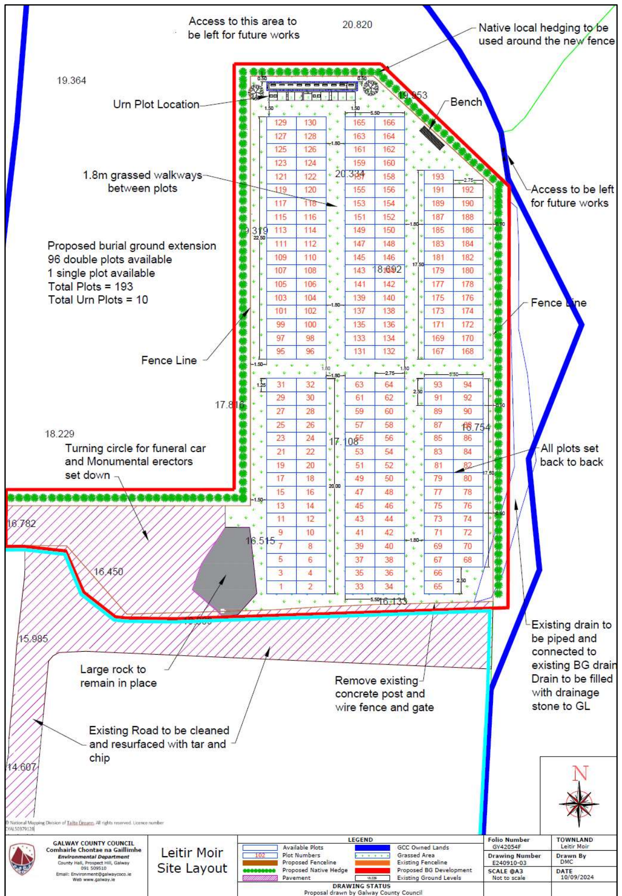
Figure 3. Plan of the Proposed Development.
