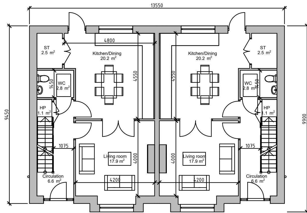
Ground Floor Plan Floor Area - 55sq.m Total Floor Area - 110sq.m
