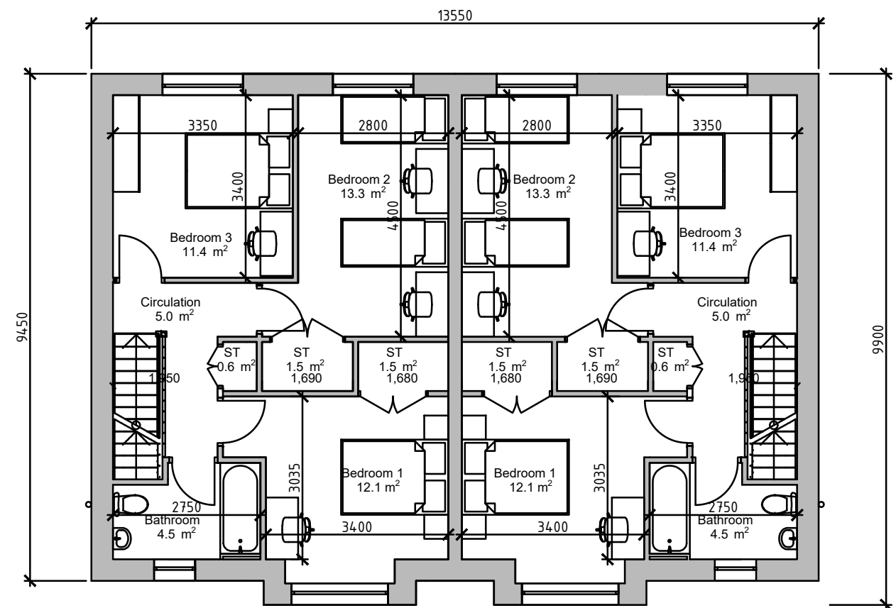
First Floor Plan Floor Area - 55sq.m
