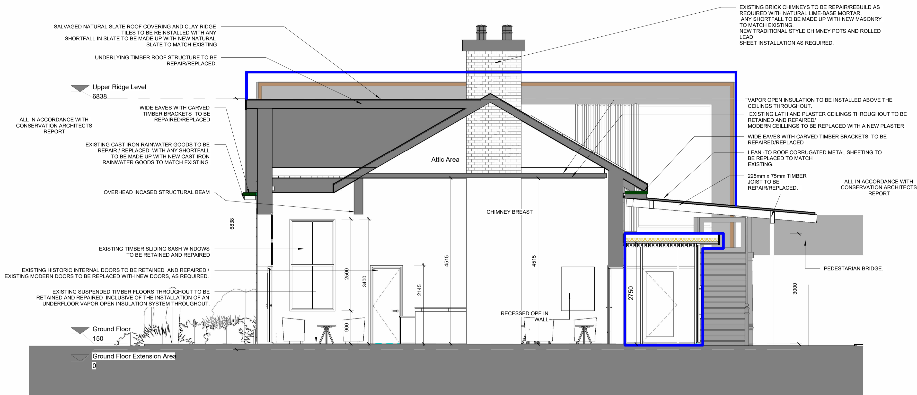
13 Section 4-Proposed 1 : 50
