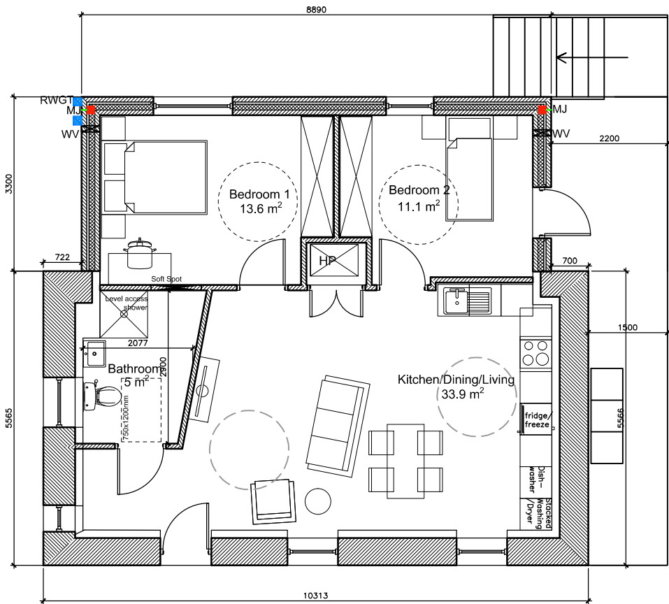
Option 1
