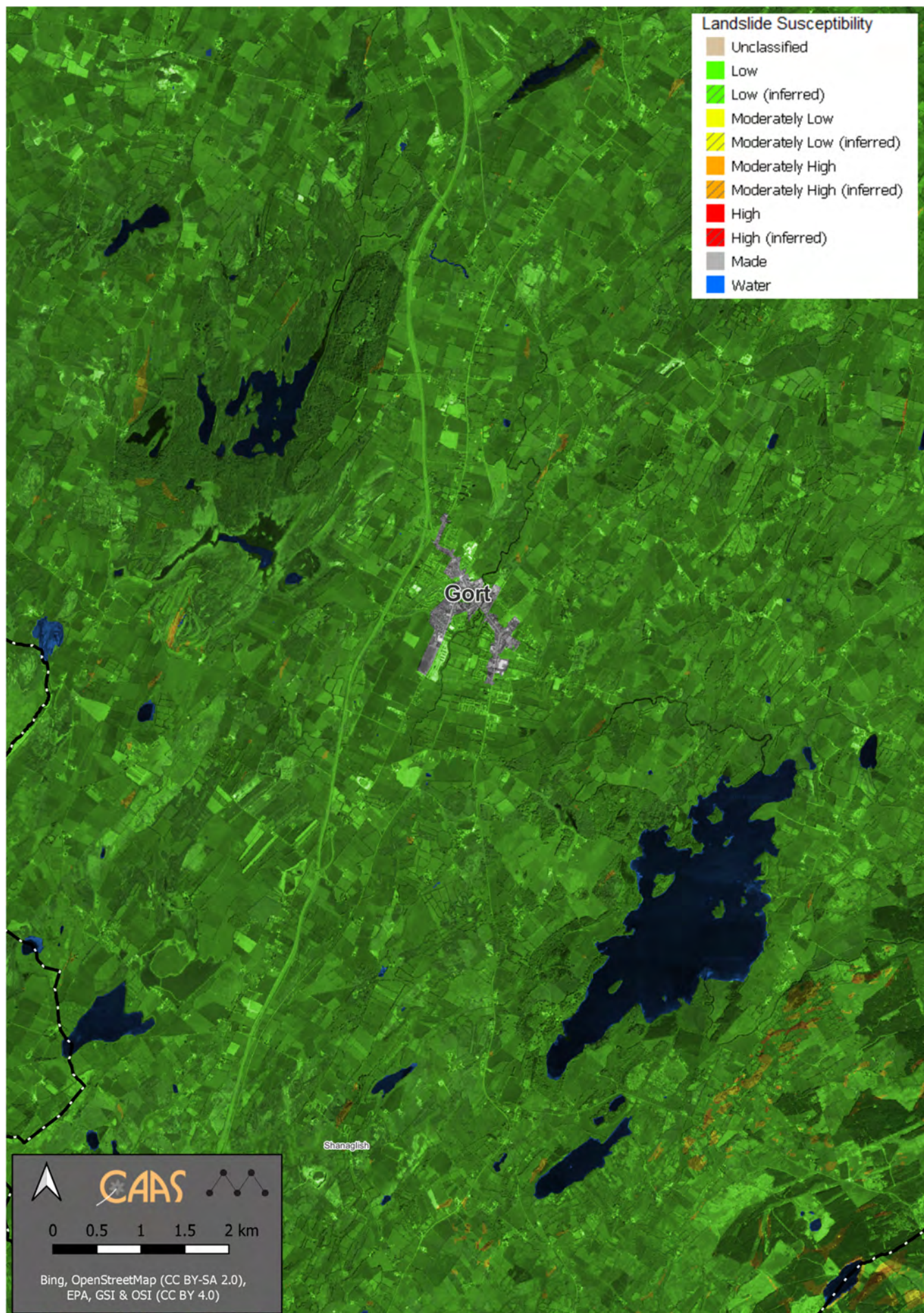
Figure 4.9 Landslide Susceptibility
