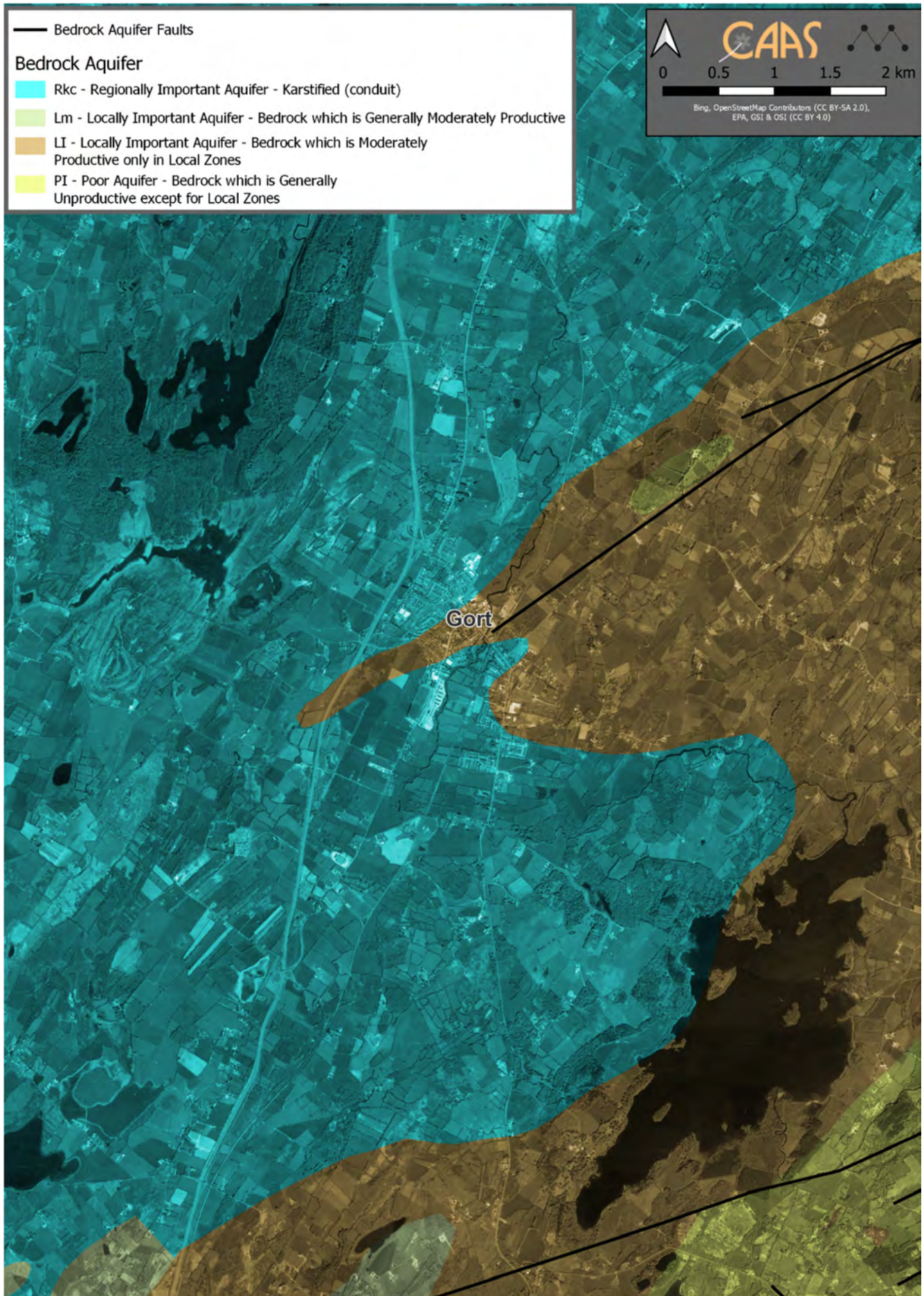
Figure 4.12 Groundwater Productivity
