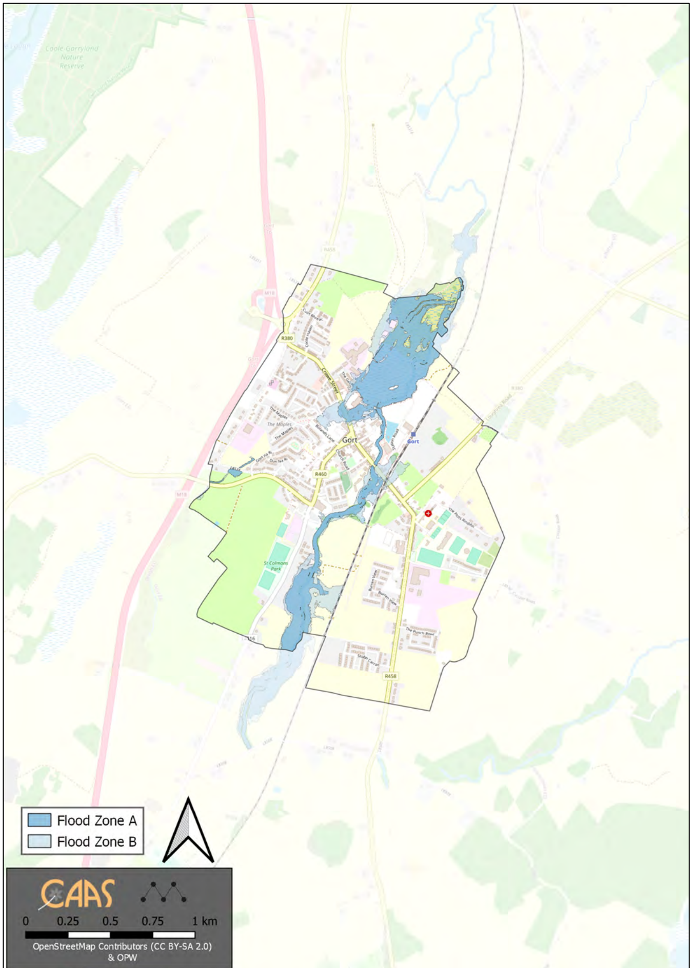
Figure 4.14 Flood Zones
