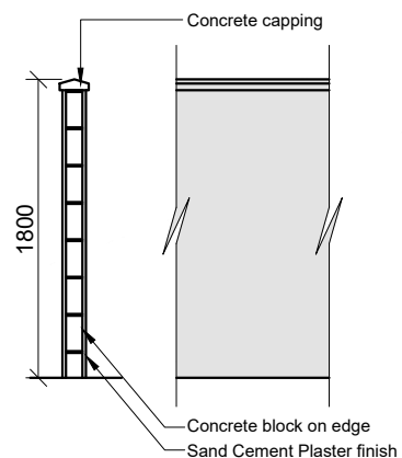
Proposed Boundary Wall Type 2
