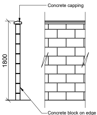
Proposed Boundary Wall Type 3
