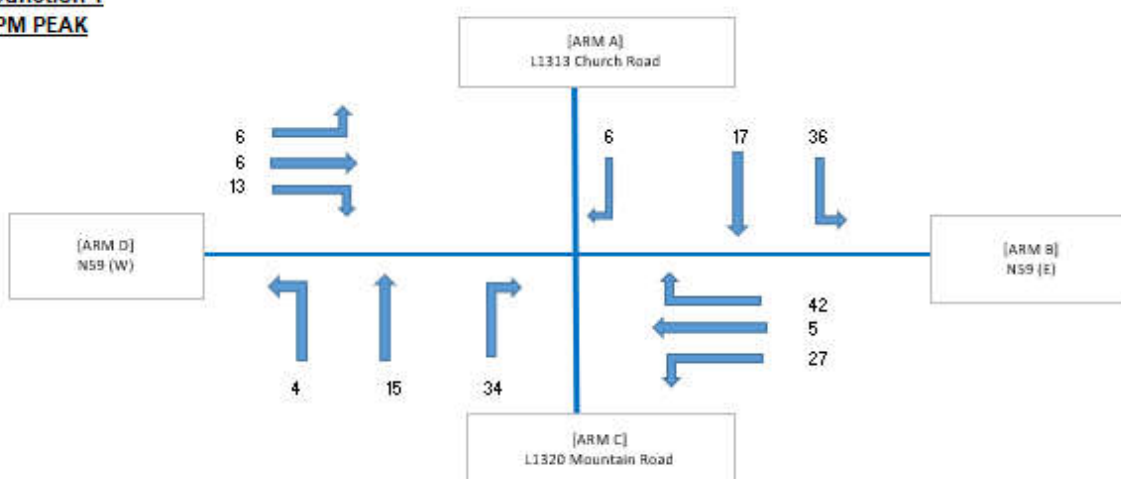
Figure 5-2 Trip Generation & Distribution Junction 1 – PM Peak
