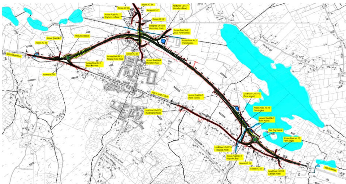
Figure 4-2: Indicative Layout Moycullen Bypass
