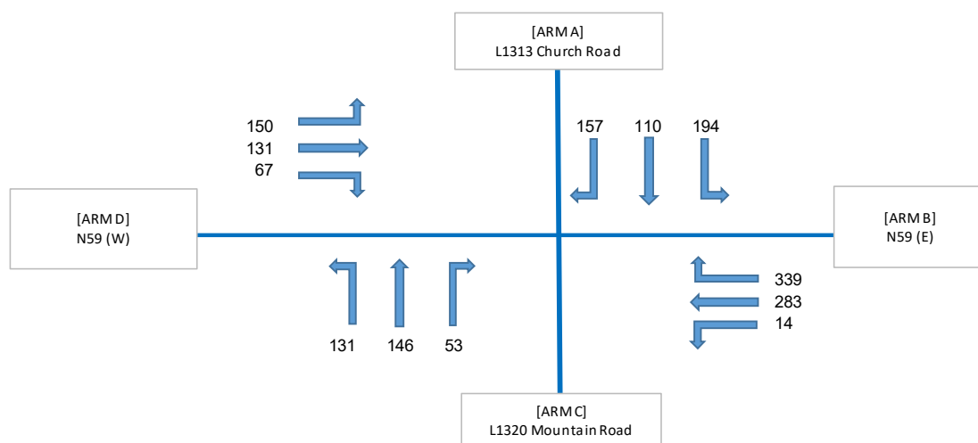
Figure 5-15 Junction 1 - 2038 PM Peak Base (With Bypass)
