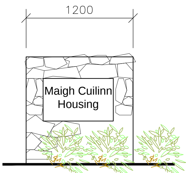
INDICATIVE ESTATE SIGNAGE; new limestone stone wall 0.6m thick and 1.2m high and 1.2m wide with stone nameplate 0.6x0.9m inset into wall foundation to Engineers details.
