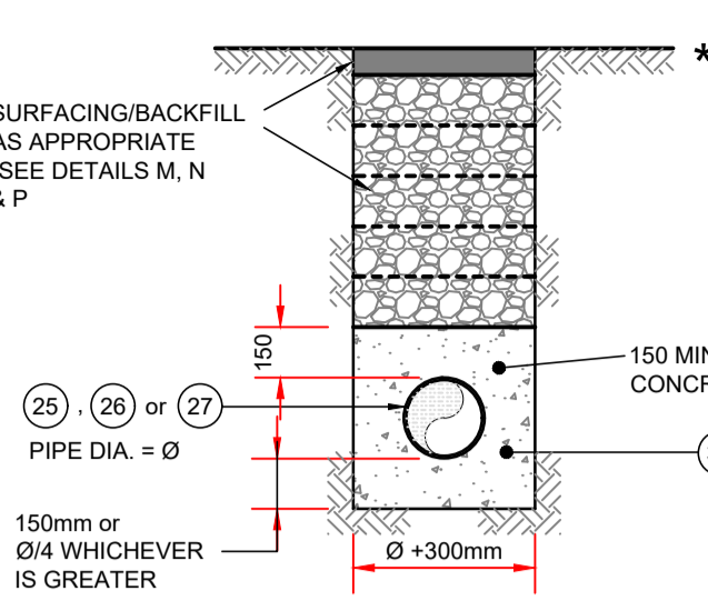
CONCRETE PIPE ENCASEMENT DETAIL
