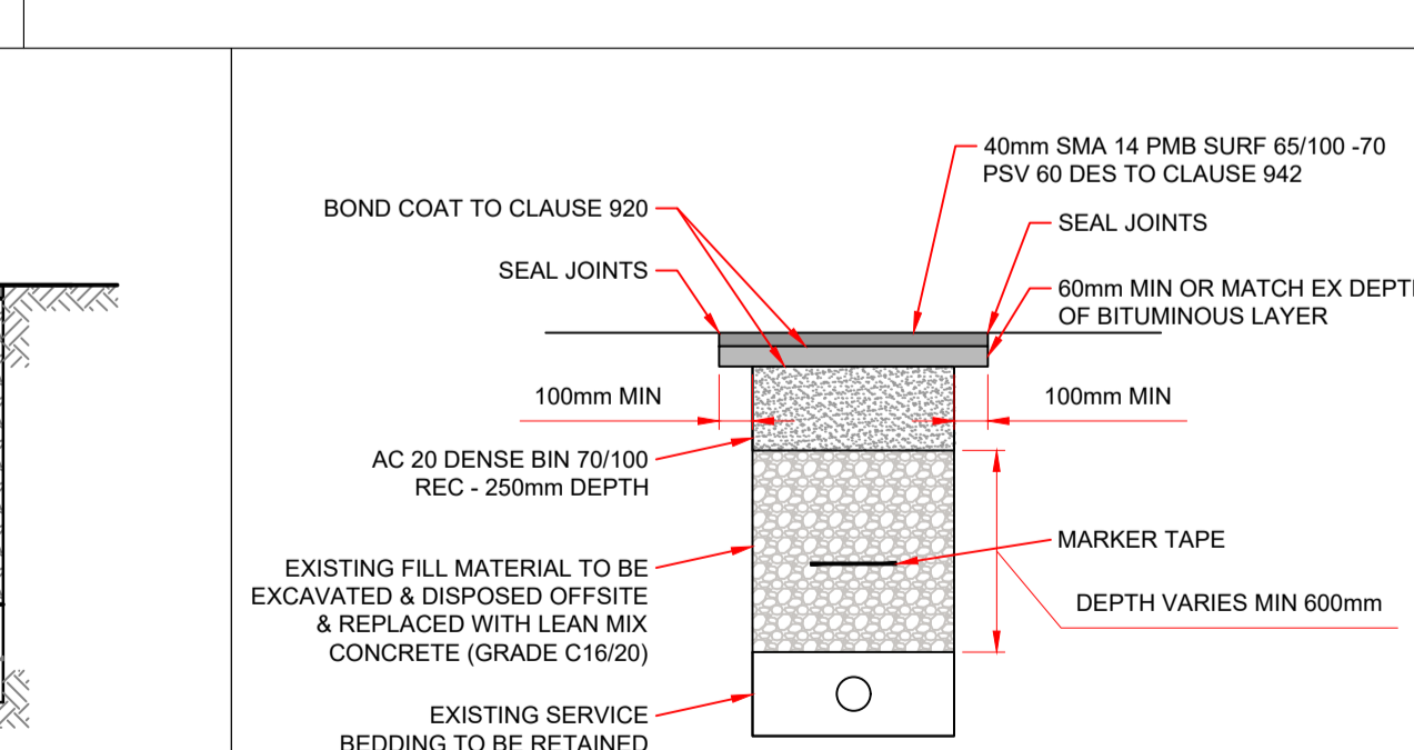
TYPICAL SERVICE REINSTATEMENT DETAIL - ASPHALT ROAD
