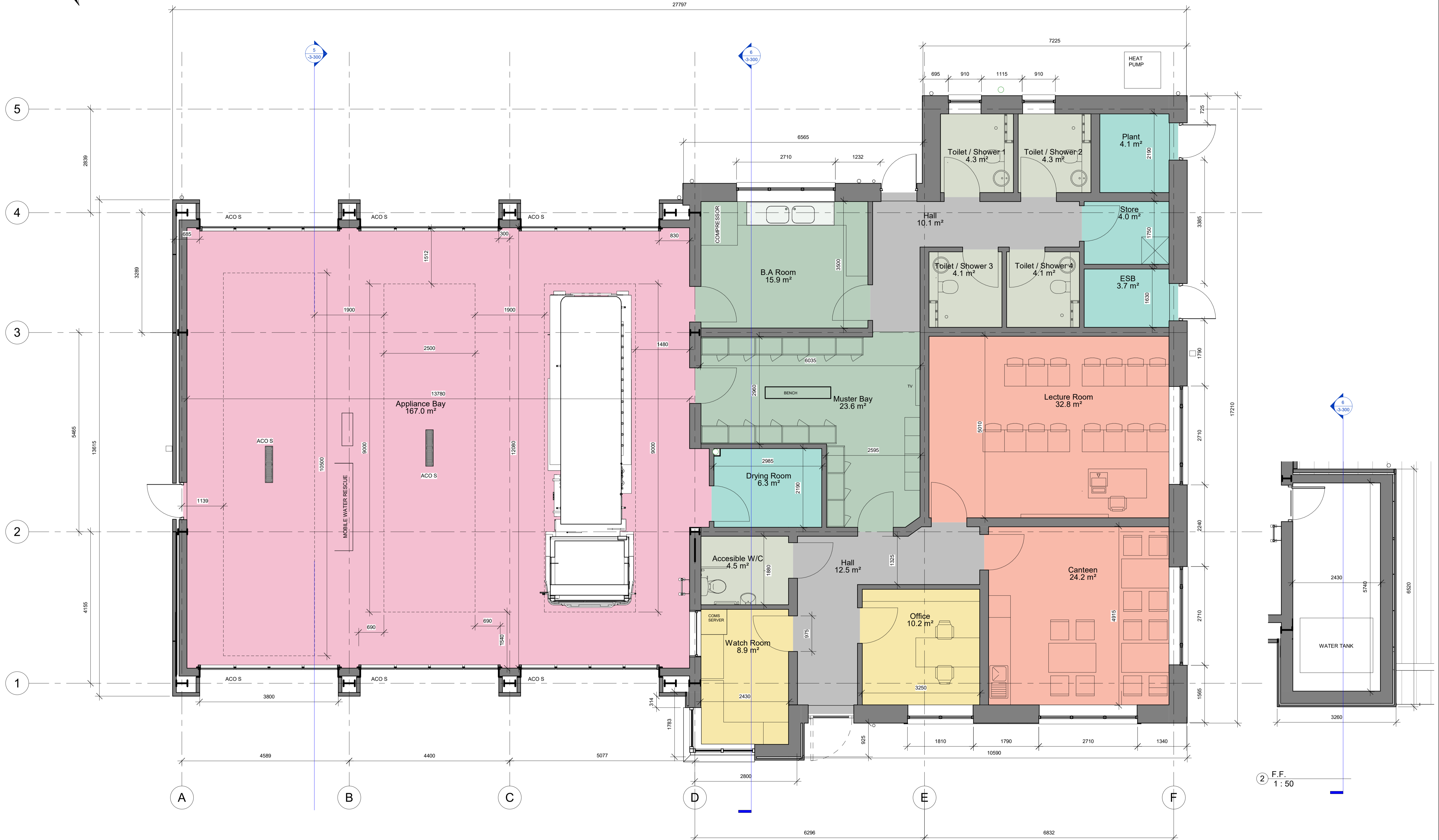
1 Ground Floor Plan 1 : 50
