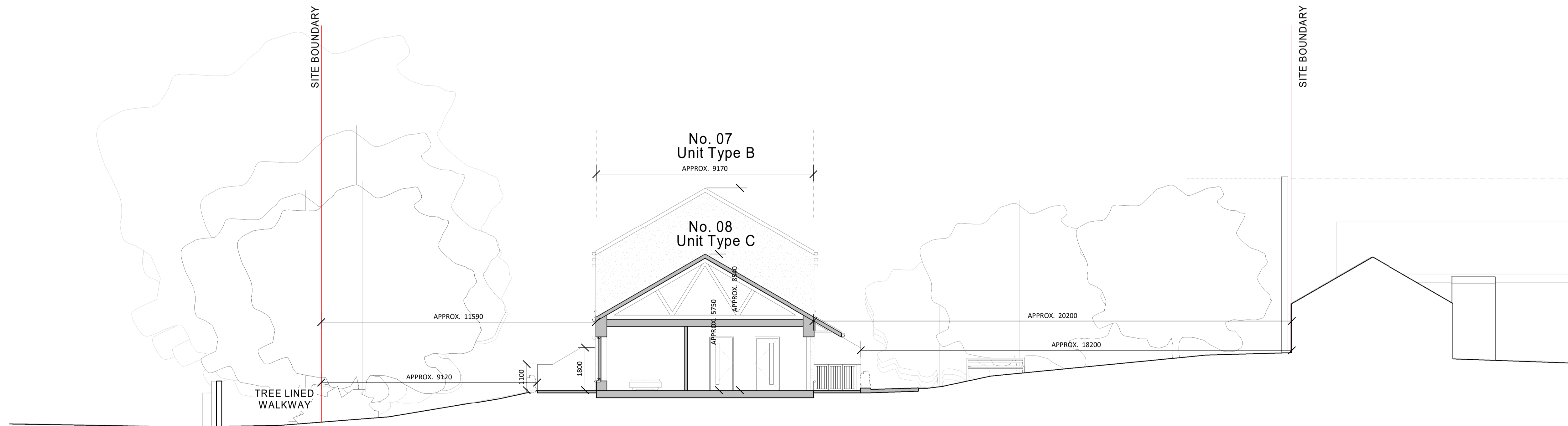
2 Unit C Section - Proposed 1 : 100
