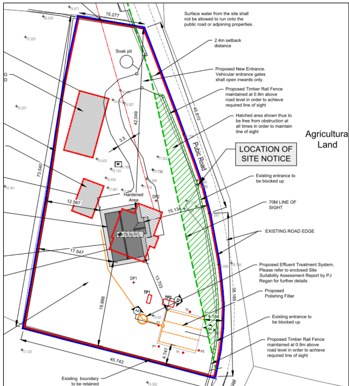
Figure 3.2: Extract of site layout drawing
