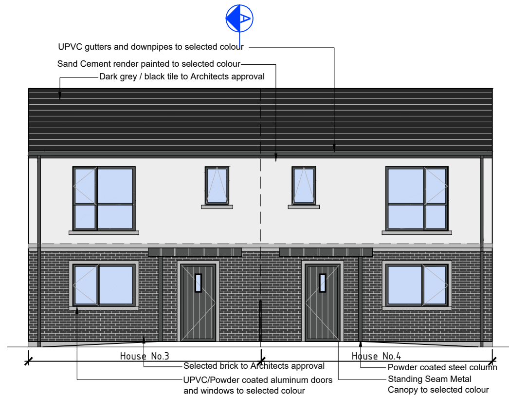
01 West Elevation
