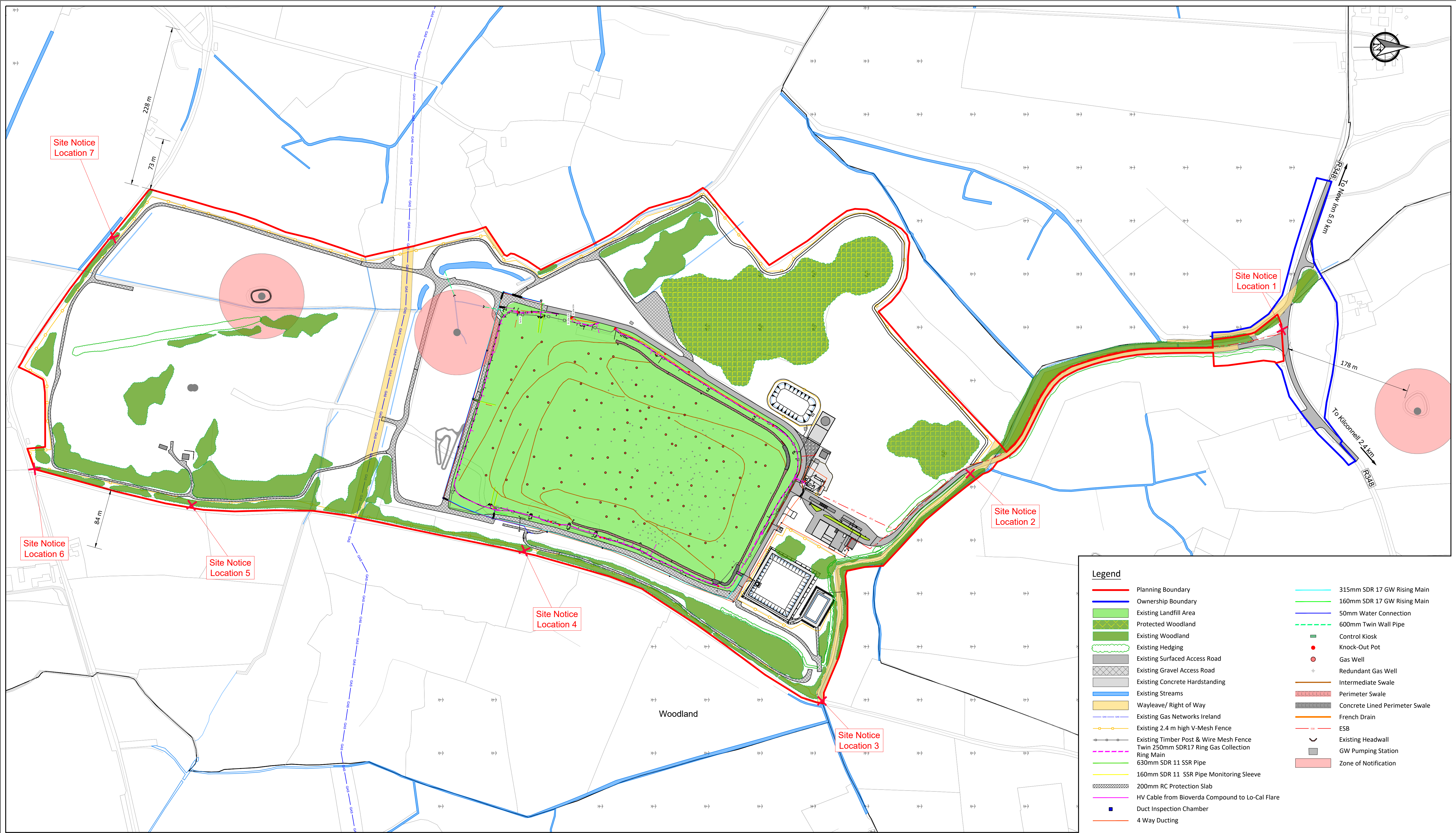
EXISTING SITE LAYOUT Scale 1:2500
