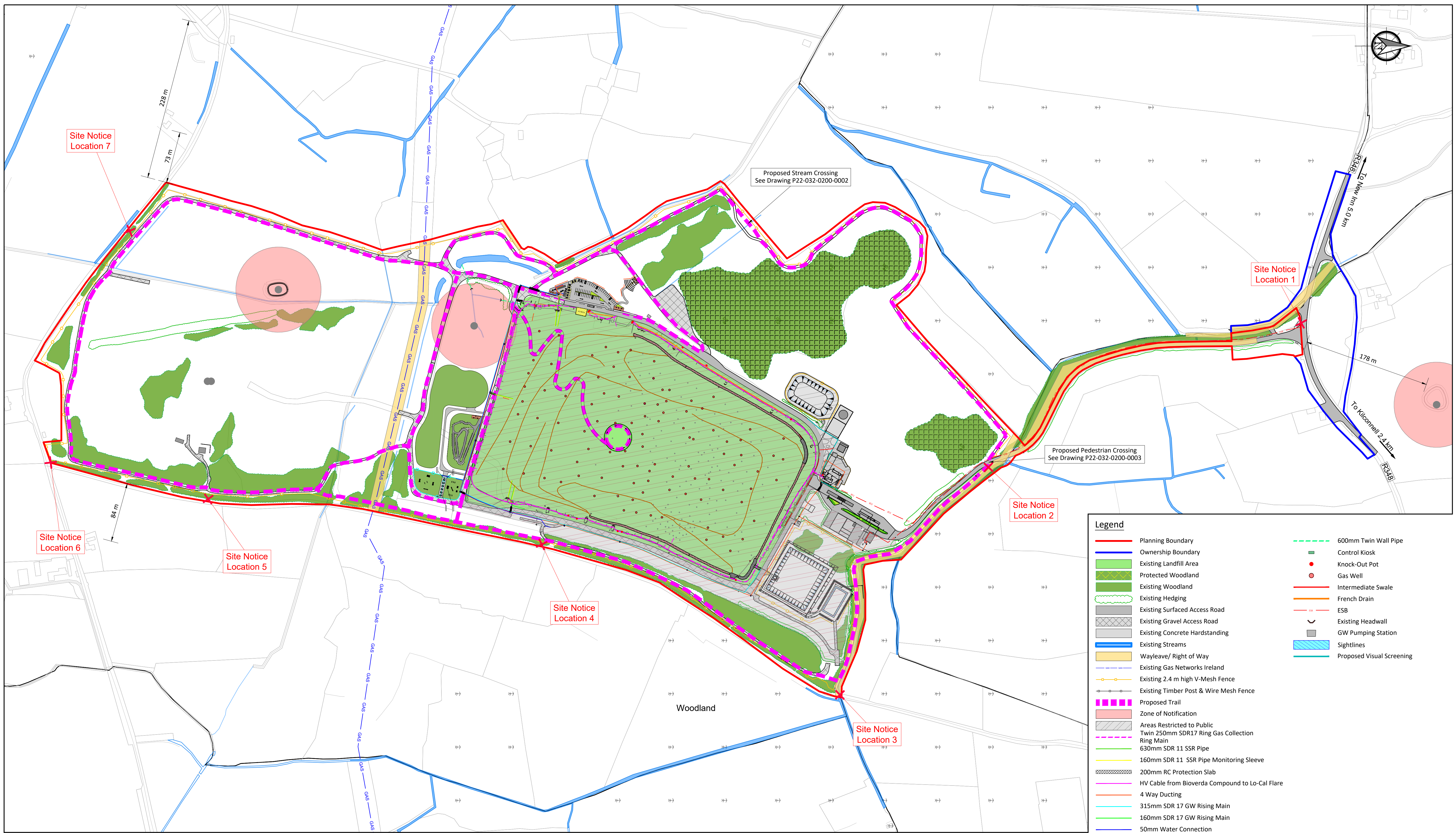
PROPOSED SITE LAYOUT Scale 1:2500
