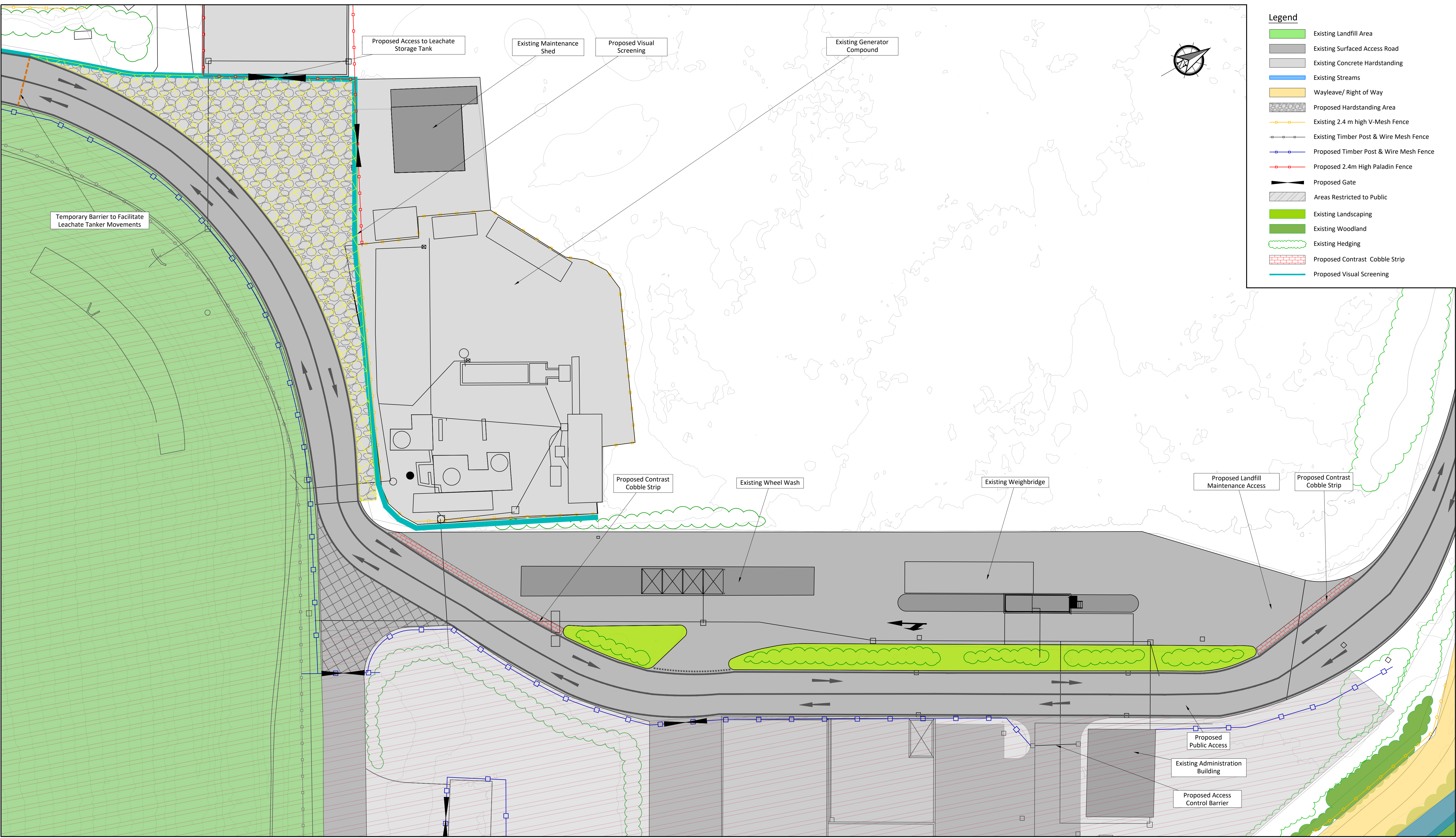
PLAN LAYOUT Scale 1:250
