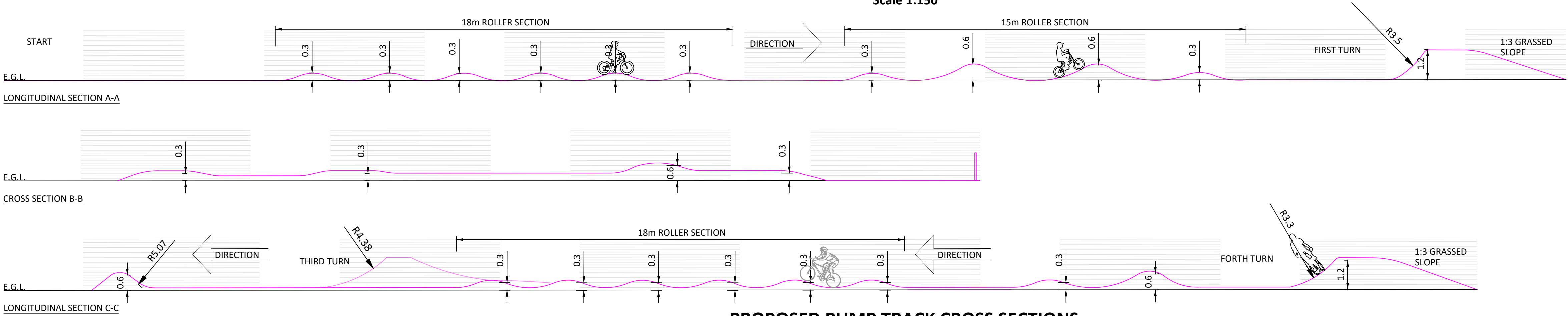
PROPOSED PUMP TRACK CROSS SECTIONS
