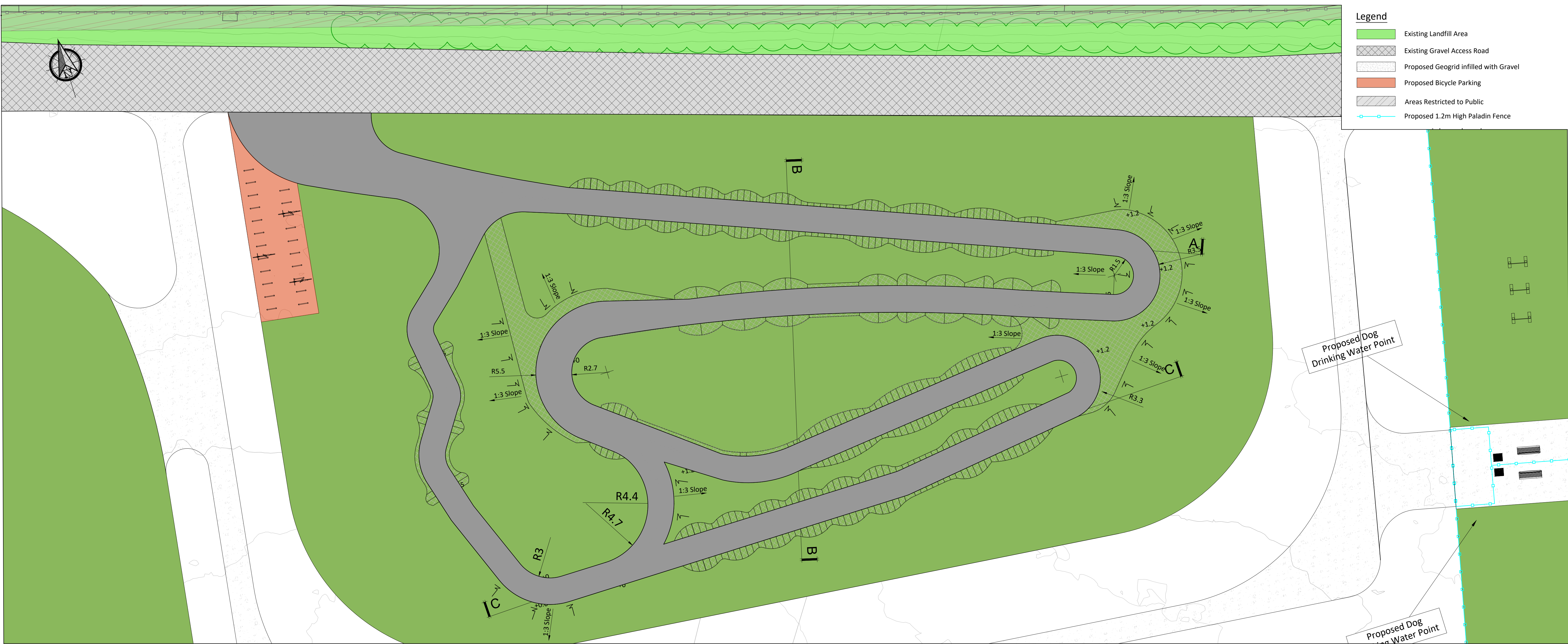
PROPOSED PUMP TRACK PLAN LAYOUT
