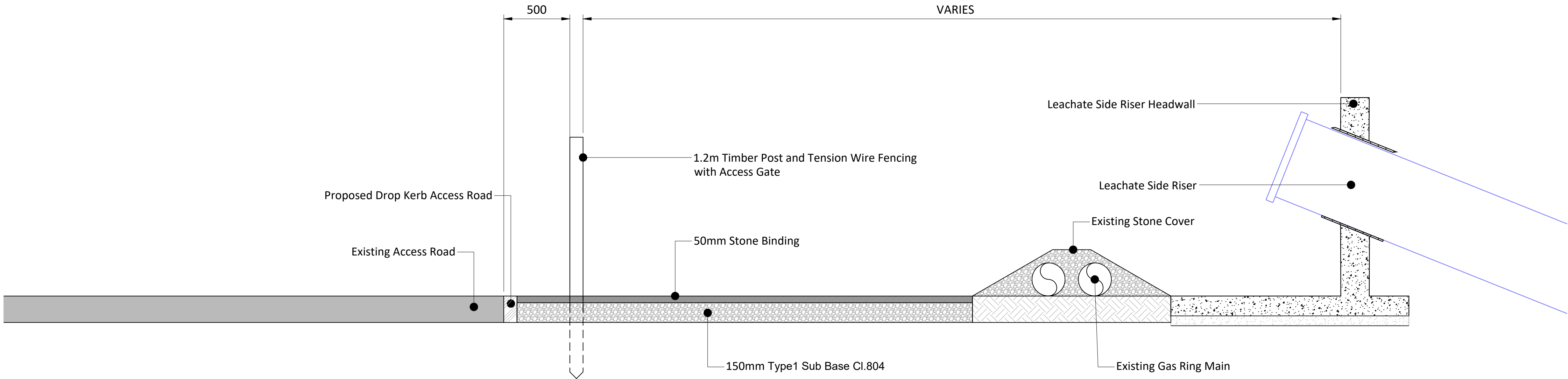
PROPOSED TYPICAL LEACHATE SIDE RISER SECTION DETAIL
