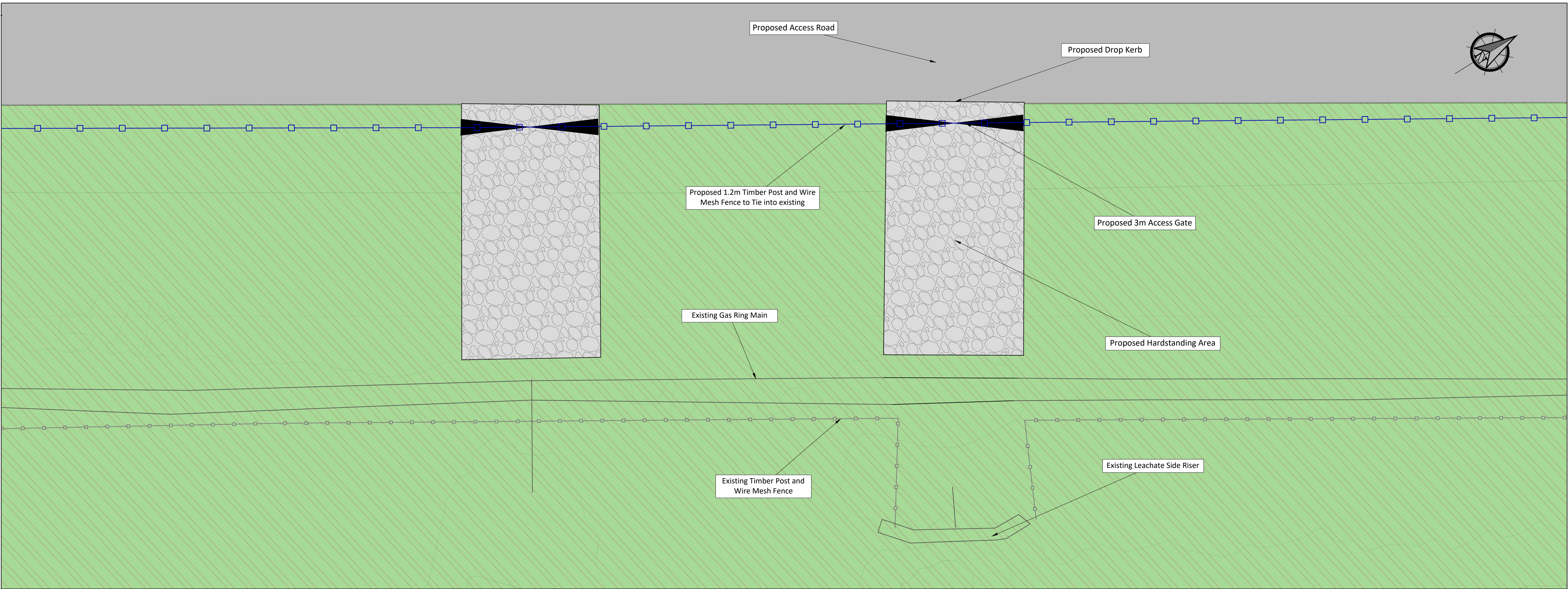
PROPOSED TYPICAL LEACHATE SIDE RISER PLAN
