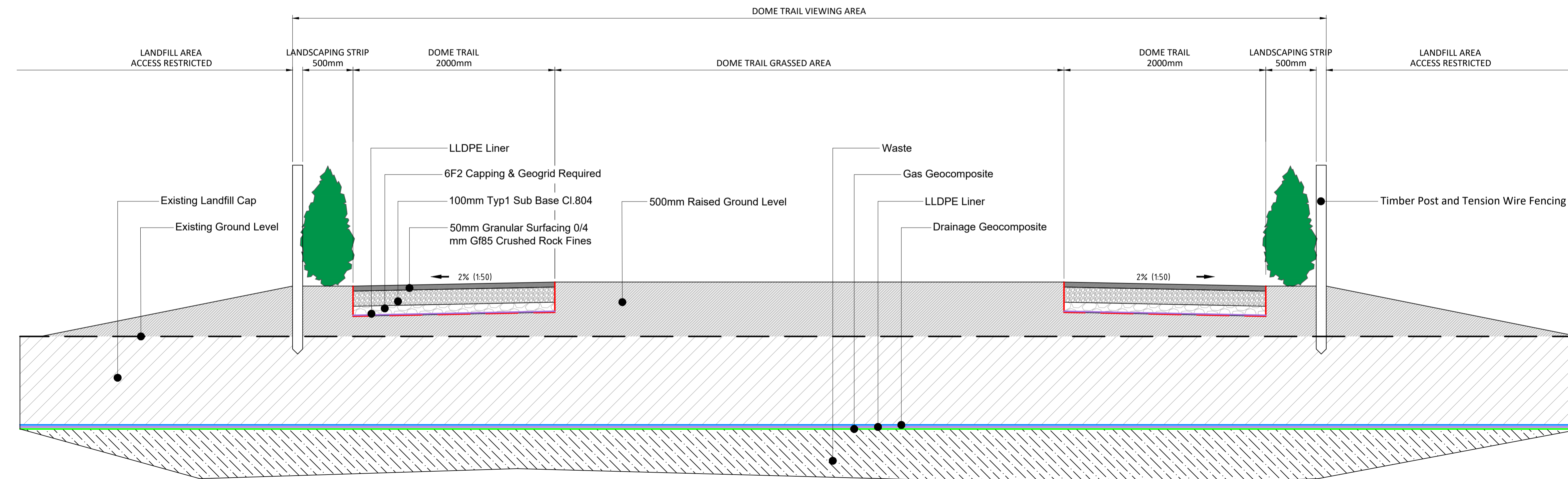
PROPOSED DOME TRAIL VIEWING AREA SECTION DETAIL Scale 1:25
