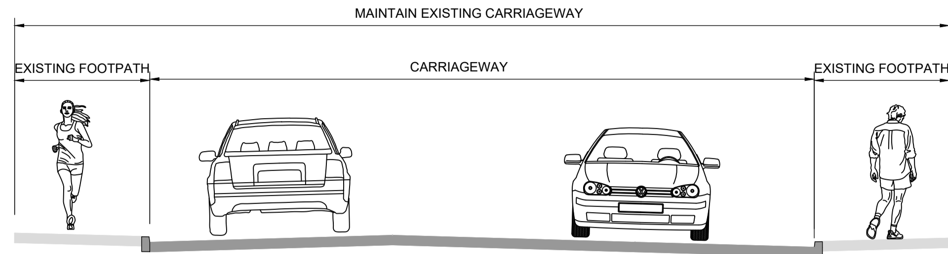
TYPICAL CROSS SECTION B-B
