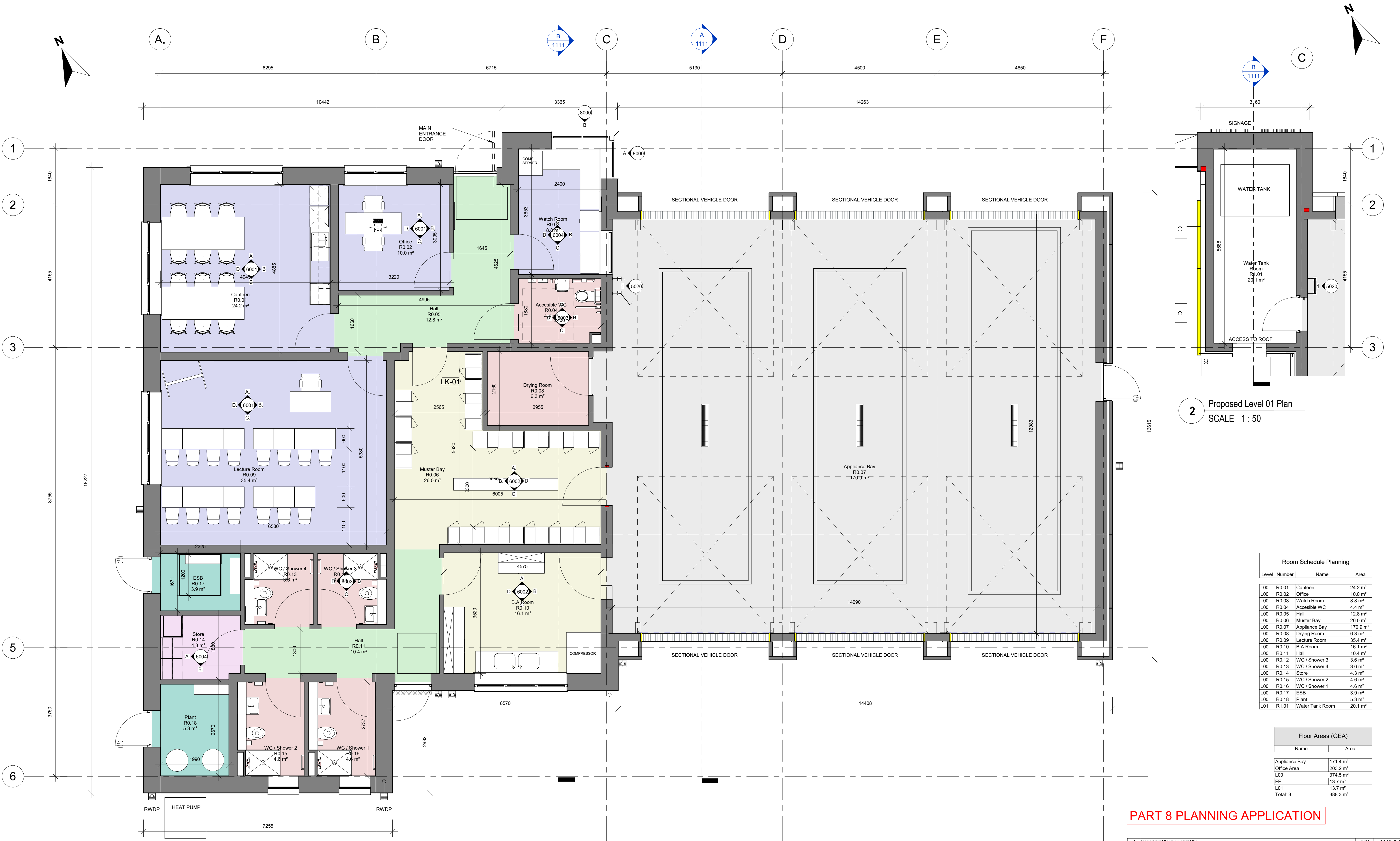
1 Proposed Ground Floor Plan SCALE 1 : 50
