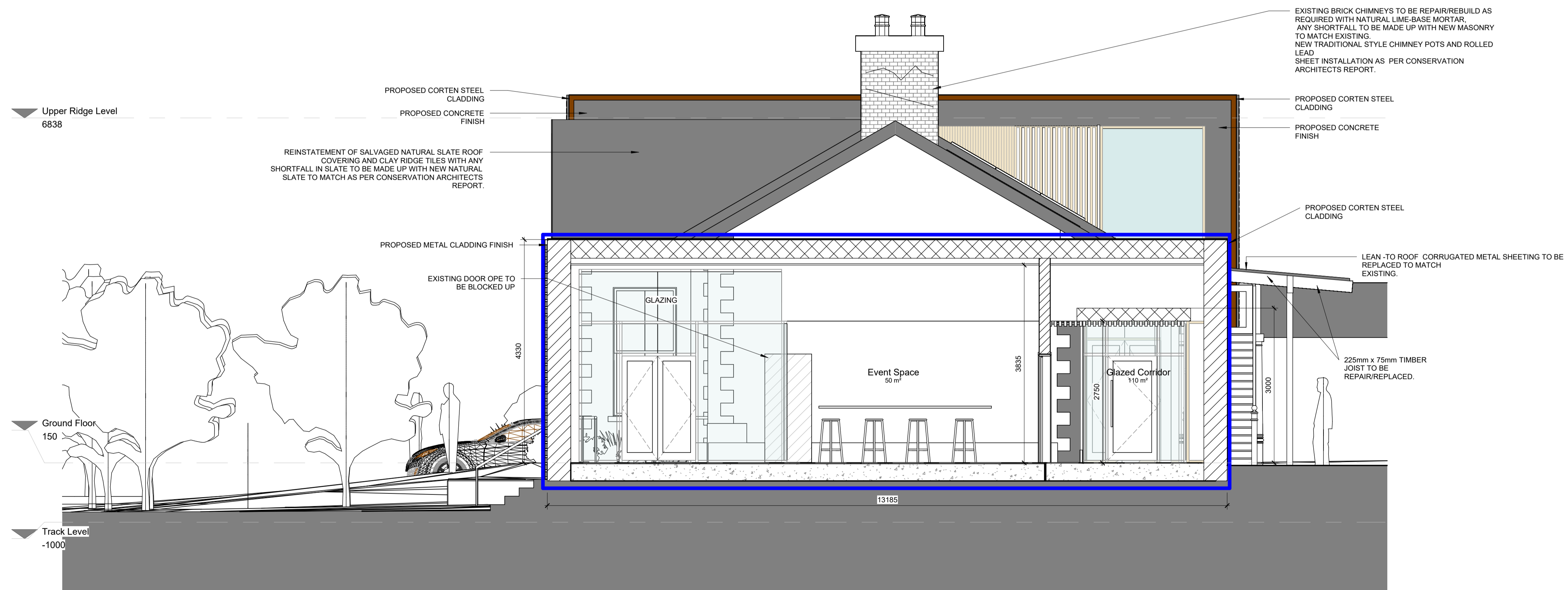
16 Proposed Section 7- Event Space 1 : 50
