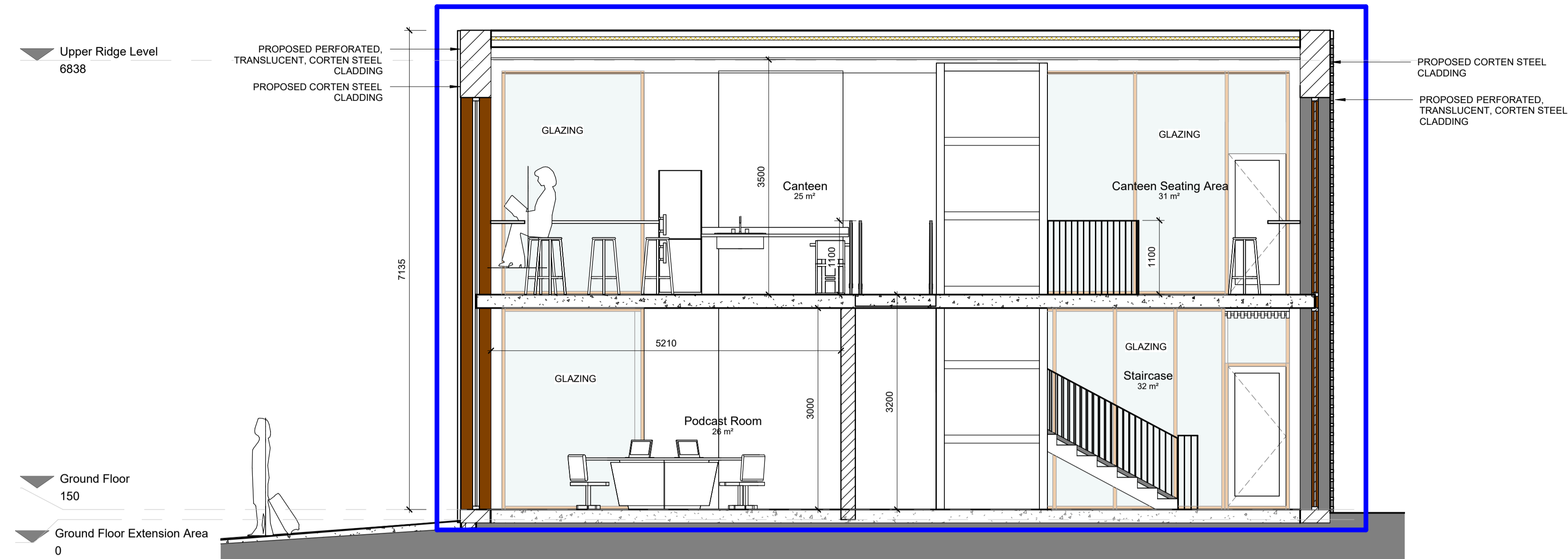
15 Proposed Section 6- Canteen and Podcast Room 1 : 50
