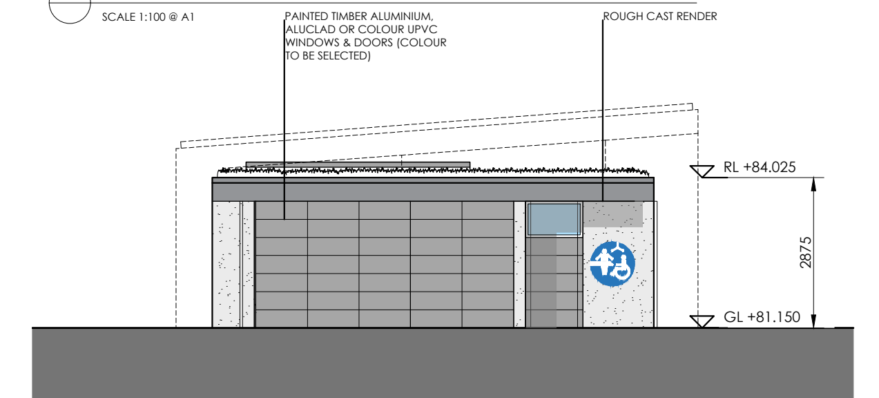
PROPOSED NORTH EAST ELEVATION - STORAGE / PLANT
